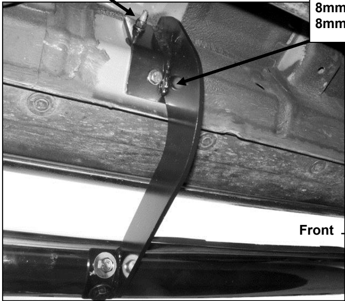
(Fig 3) Driver side center mounting location pictured
