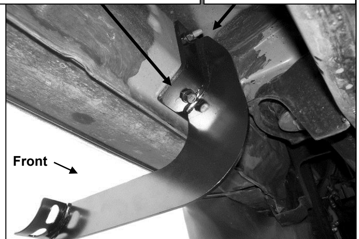
(Fig 2) Driver side front mounting location
